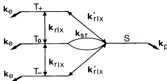
Fig. 6. Scheme for biradical reactions. Rate constants for the following processes: k_{\text{rel}} , spin-lattice relaxation among triplet sublevels; k'_{\text{rel}} , spin-lattice relaxation between T_+ ( T_- ) and S states; k_{\text{ST}} , intersystem crossing between T_0 and S states; k_e , bimolecular escape process (intermolecular biradical decay process); k_p , unimolecular cage product formation.
