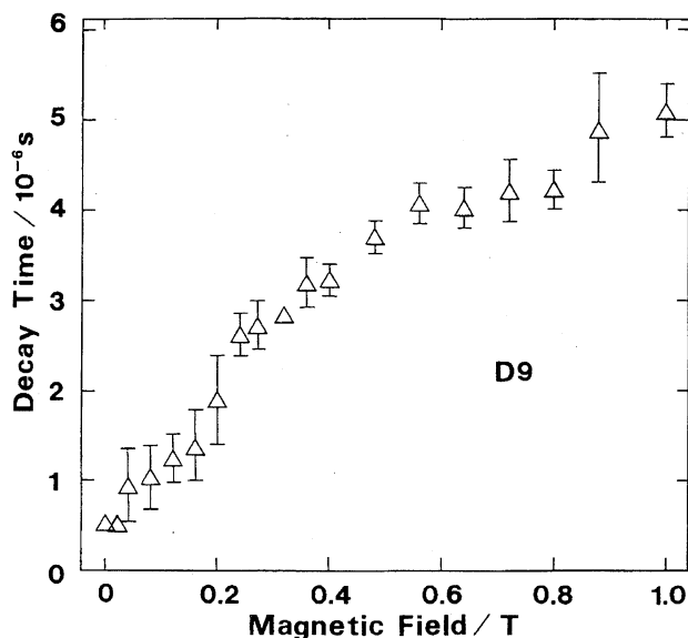
Fig. 5. Magnetic field effects on the decay time for biradical derived from D9.
