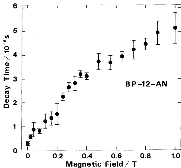
Fig. 1. Magnetic field effects on the decay time for biradical derived from BP-12-AN.
