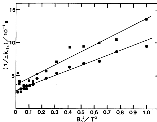
Fig. 7. Plot of (\Delta k_{\text{rel}})^{-1} against B_0^2 . Circles for biradical derived from \alpha 13, squares for biradical derived from 13BP.
