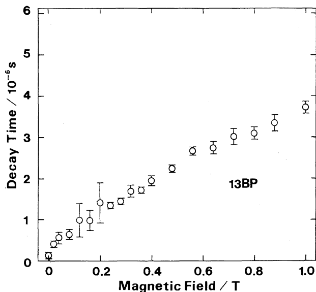
Fig. 2. Magnetic field effects on the decay time for biradical derived from 13BP.
