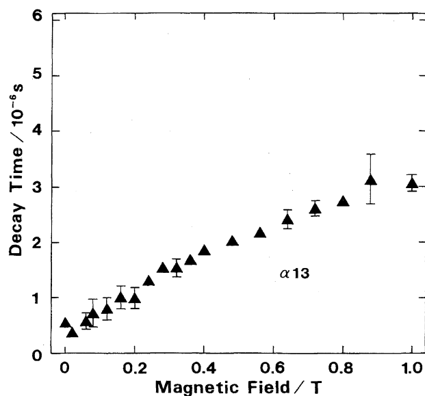
Fig. 3. Magnetic field effects on the decay time for biradical derived from \alpha 13.
