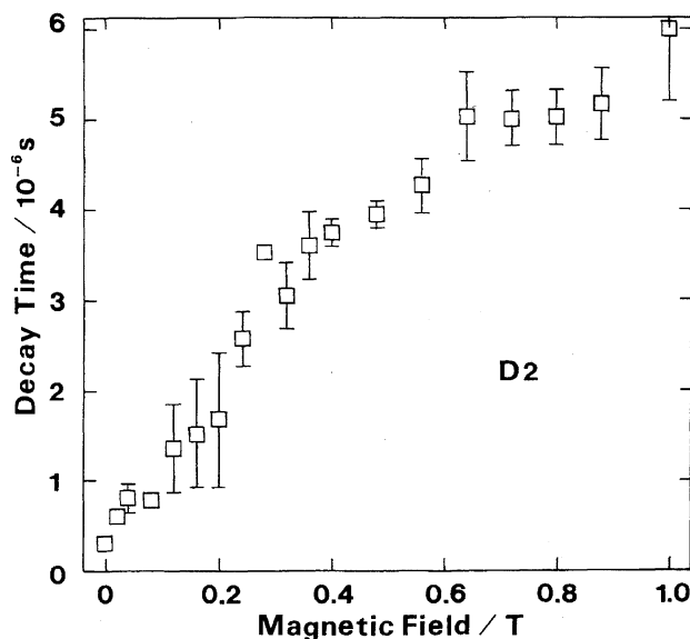
Fig. 4. Magnetic field effects on the decay time for biradical derived from D2.
